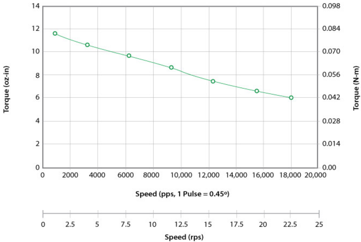
ZN417-11-03 (0.9° Step Motor) 24VDC, 1.68 Amp Peak, Bipolar, 1/2 Stepping
